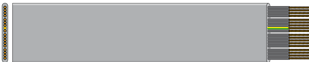
Drawing according to part number 148 779 – Type 6777-F
