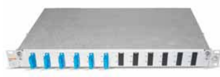
Fibre optic breakout box OV-A, 19"/1U, extractable, configuration example with 6 SCD adapters, without pigtails
