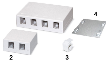
2 Surface Mount Box for 2 or 4 Keystone modules without dust shutters 3 Blank cover for unused ports 4 Mounting plate
