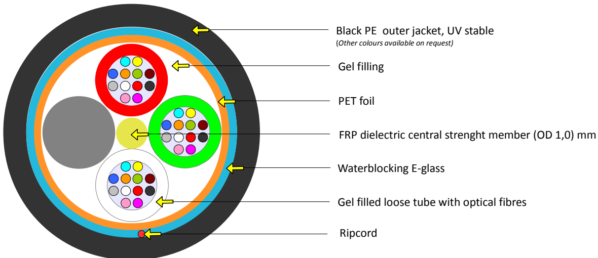
The picture represents a cable with 36 optical fibres
