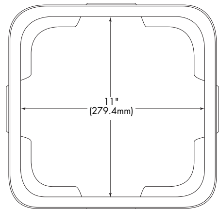
GLB1111 Grade Level Box Interior Dimensions
